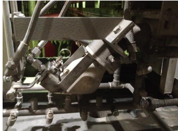
Teflon cleaning head for Dryer Fabric cleaning with HP water and passivation fluid
